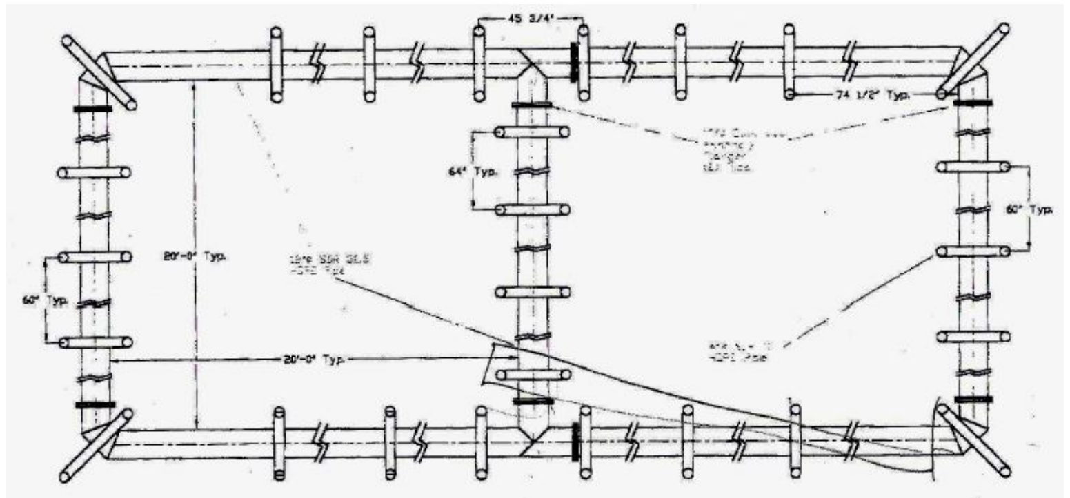
Figure 2. Typical Drawing of current Net Pens.
