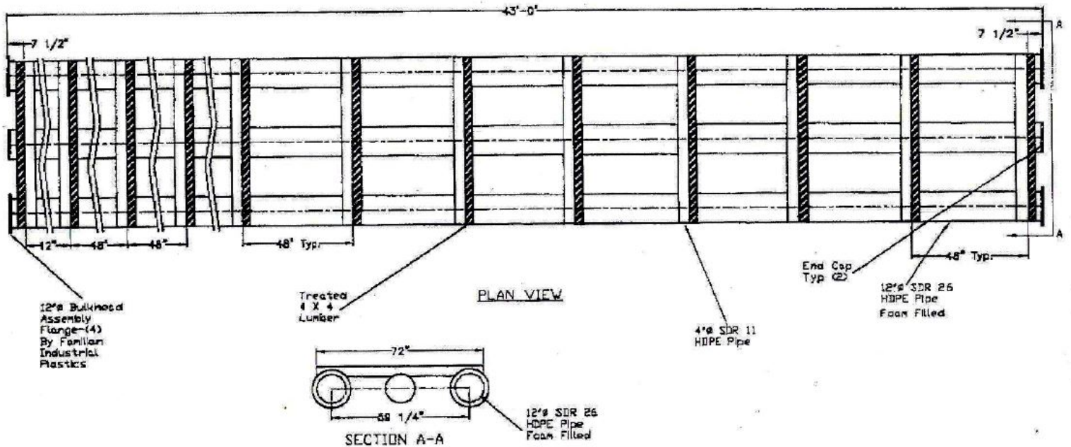
Figure 1. Drawing of Typical Dock.
